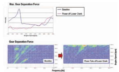
Figure 5: Solution for Gear Resonance: Power Take-off Moved to Lower Crankshaft
