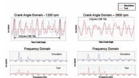
Figure 6: Correlation of Crank Nose Speed Fluctuation
