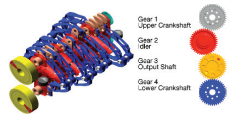
Figure 1: Adams/Engine Crank Train model with Flexible Components and Rear View
