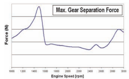
Figure 3: Maximum Gear Separation Force Over Engine Speed
