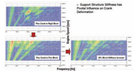
Figure 2: Support Structure Sensitivity, Influence on Crank Bending
