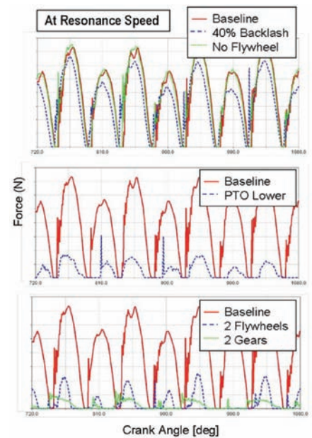
Figure 4: Selected Solutions of the Gear Resonance Mitigation Study
