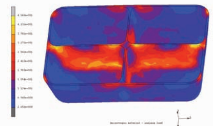
Figure 10: As-Molded (Anisotropic) Material Model
